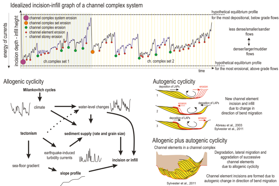
Fig. 10. Idealized incision-infill graph showing hierarchies from channel storeys to channel complex system and possible allogenic and autogenic controls on incision-infill cycles (Tókes et al., 2021, this VSI). LAP = Lateral Accretion Package, ch. = channel.
